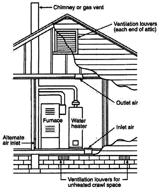
FIGURE 5-9 All Combustion Air from Outdoors - Inlet Air from Ventilated Crawl Space and Outlet Air to Ventilated Attic.
