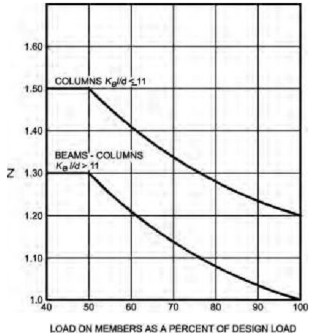
FIGURE 721.6.3(1) LOAD FIGURE
