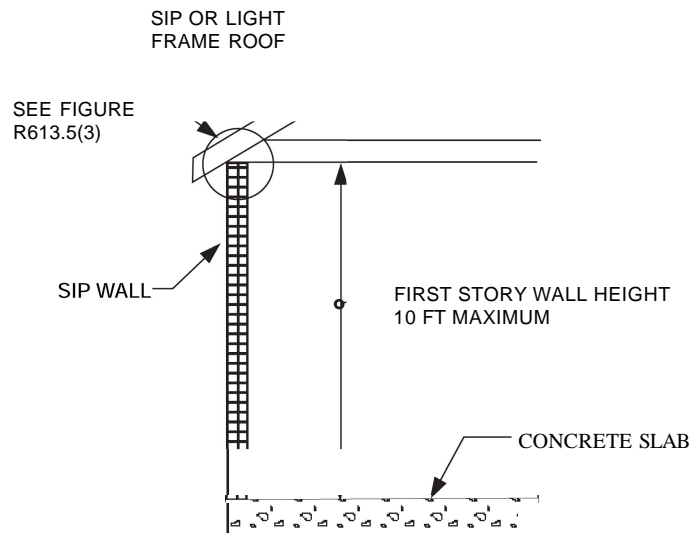
FIGURE R613.5(1) MAXIMUM ALLOWABLE HEIGHT OF SIP WALLS
