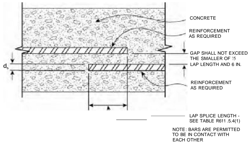
FIGURE R611.5.4(1) LAP SPLICES
