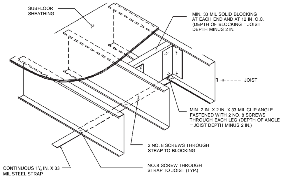
FIGURE R505.3.3.2(1) JOIST BLOCKING (SOLID)
