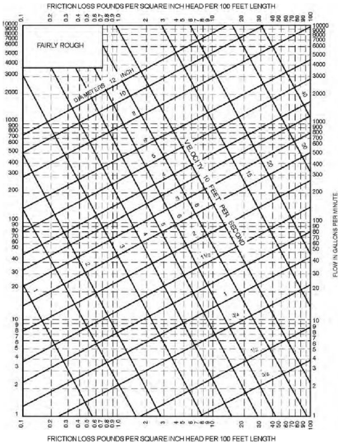
FIGURE AP103.3(6) FRICITION LOSS IN FAIRLY ROUGH PIPE a
