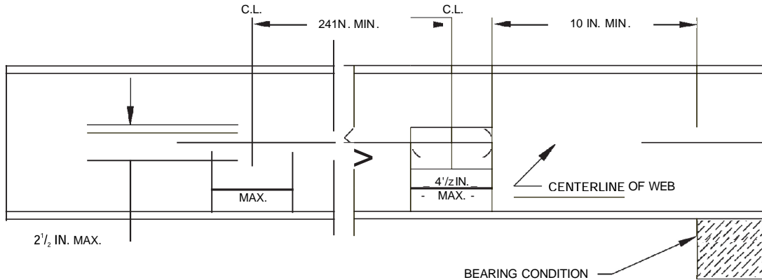
FIGURE R505.2.5.1 FLOOR JOIST WEB HOLES
