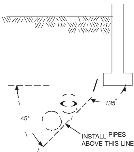
FIGURE P2604.4 PIPE LOCATION WITH RESPECT TO FOOTINGS
