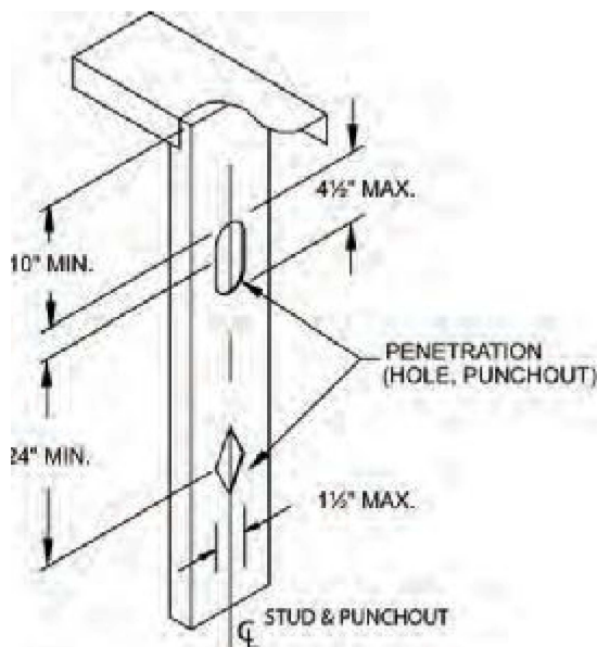
FIGURE R603.2.5.1 WEB HOLES
