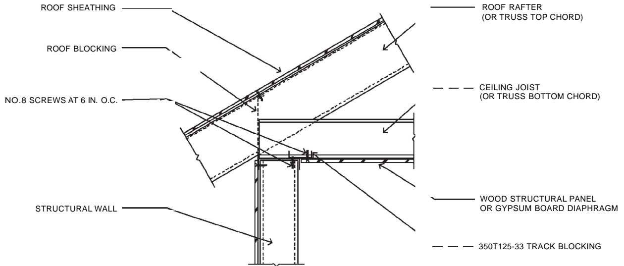
FIGURE R804.3.8(2) CEILING DIAPHRAGM TO SIDEWALL DETAIL
