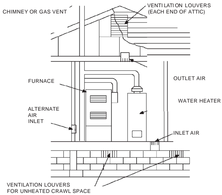
FIGURE G2407.6.1(1) [304.6.1(1)] ALL AIR FROM OUTDOOR-INLET AIR FROM VENTILATED CRAWL SPACE AND OUTLET AIR TO VENTILATED ATTIC (see Section G2407.6.1)
