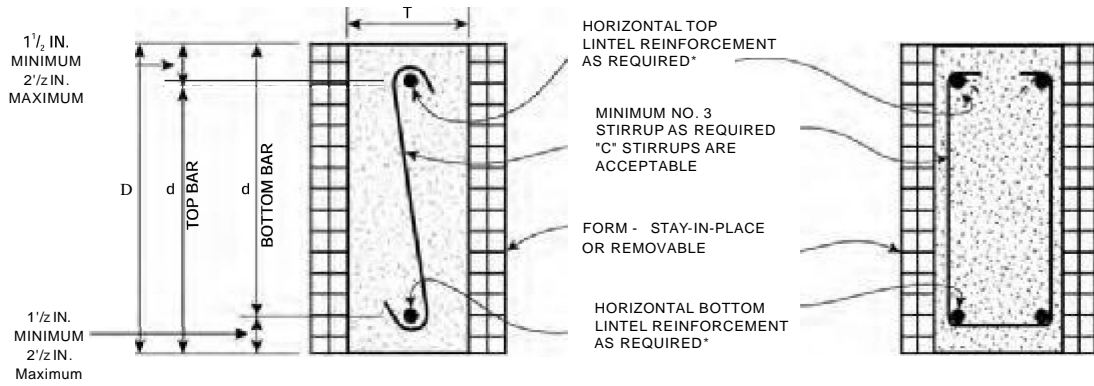
FIGURE R611.8(2) LINTEL FOR FLAT WALLS
