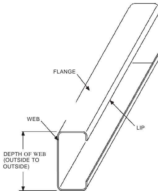
FIGURE R603.2(1) C-SHAPED SECTION
