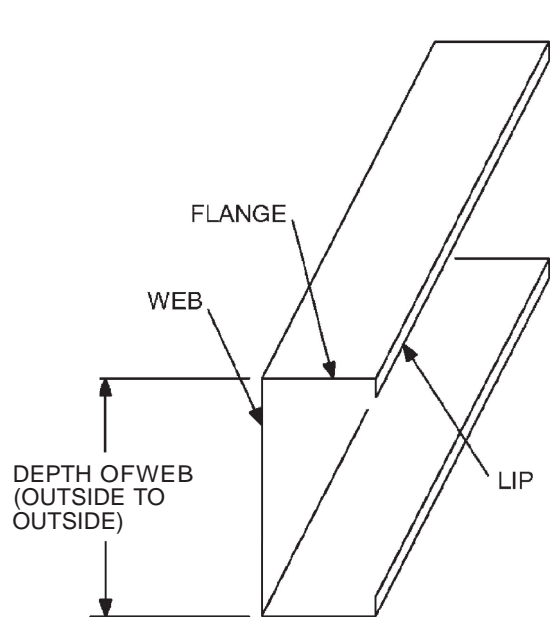
FIGURE R505.2(1) C-SHAPED SECTION
