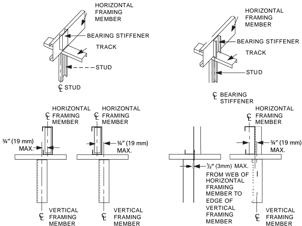
FIGURE R603.1.2 IN-LINE FRAMING
