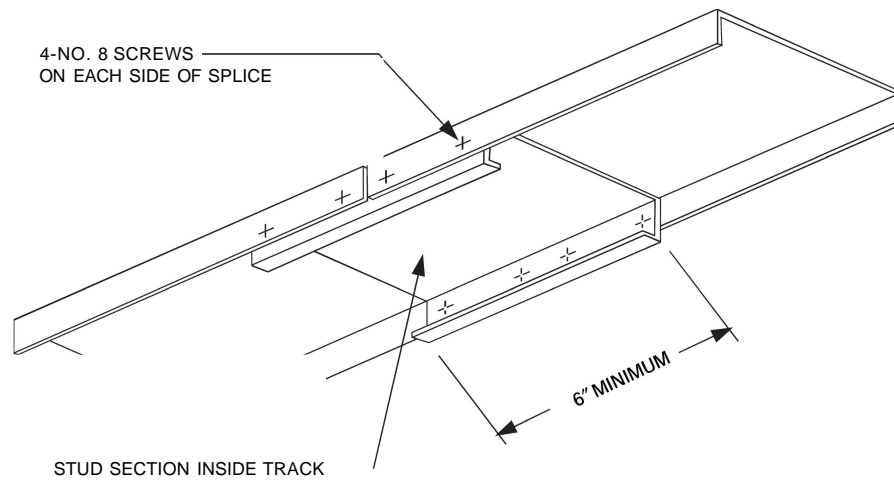
FIGURE R603.3.5 TRACK SPLICE
