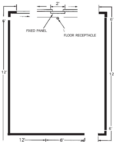
FIGURE E3901.2 GENERAL USE RECEPTACLE DISTRIBUTION
