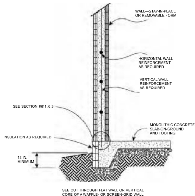
SECTION CUT THROUGH FLAT WALL OR VERTICAL CORE OF A WAFFLE- OR SCREEN-GRID WALL
