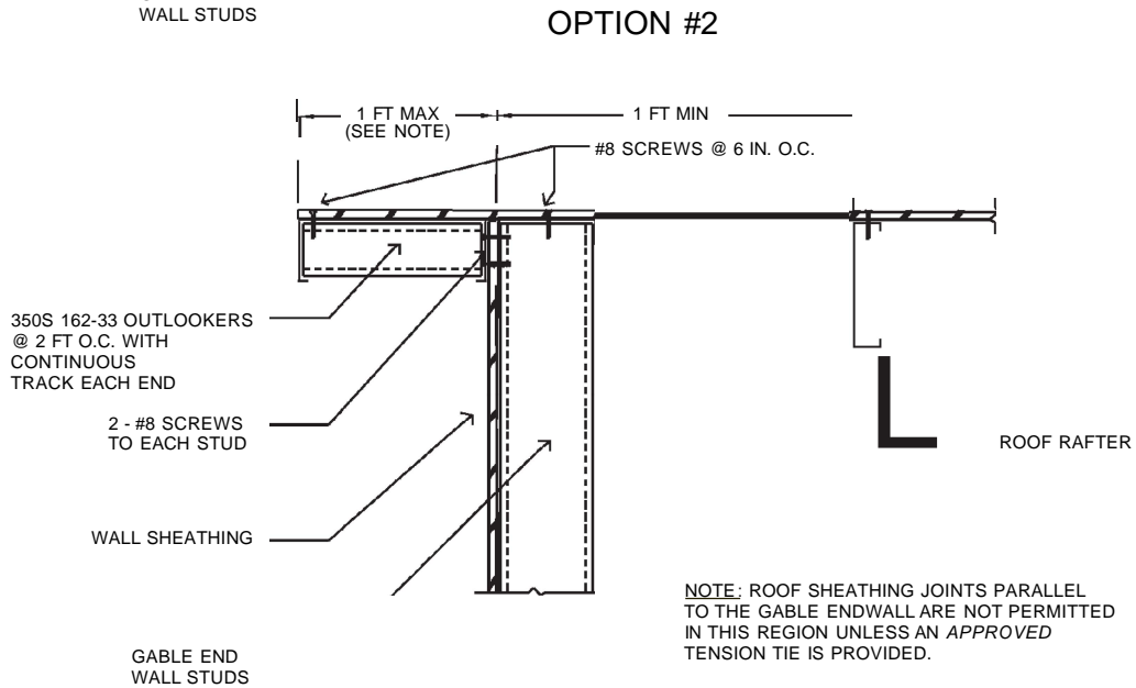
FIGURE R804.3.2.1.2 GABLE ENDWALL OVERHANG DETAILS
