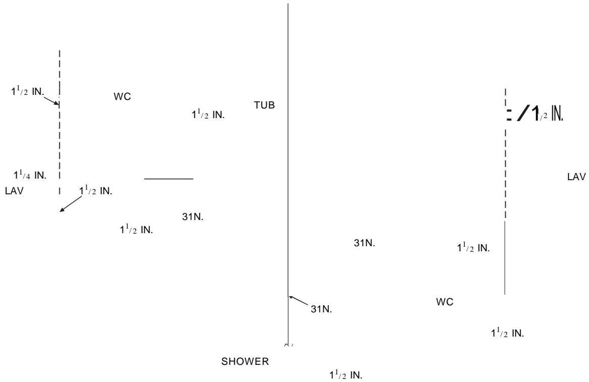
B. HORIZONTAL WET VENTING
