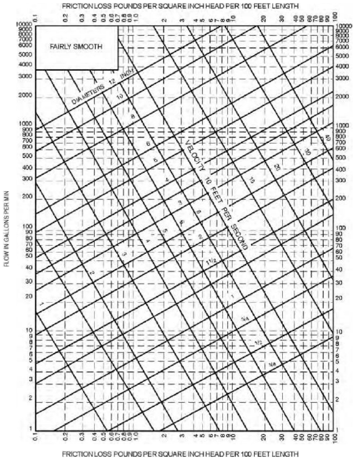
FIGURE AP103.3(5) FRICTION LOSS IN FAIRLY SMOOTH PIPE a
