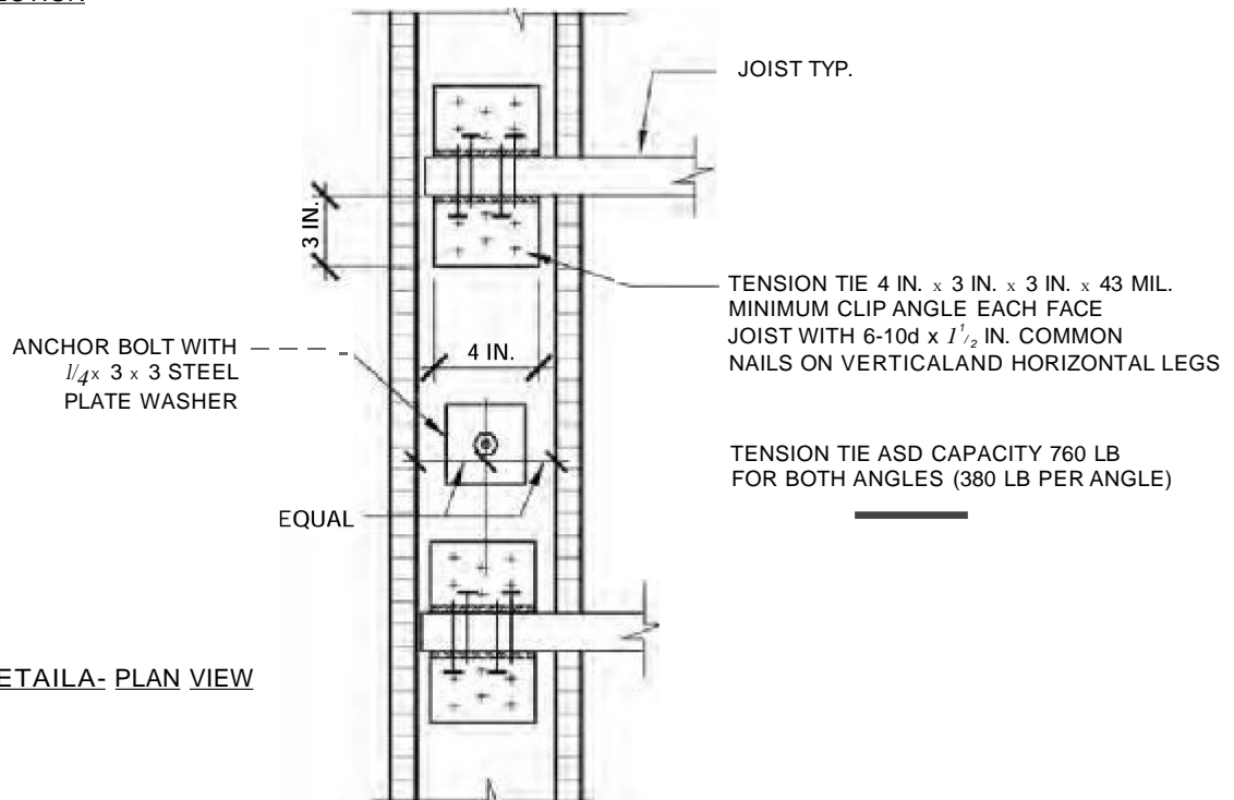
FIGURE R611.9(3) WOOD FRAMED FLOOR TO TOP OF CONCRETE WALL FRAMING PERPENDICULAR
