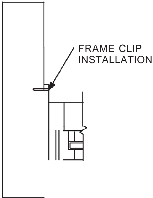
FIGURE R612.8(2) FRAME CLIP
