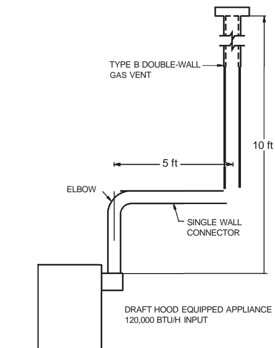
FIGURE B-15 (EXAMPLE 1) SINGLE DRAFT-HOOD-EQUIPPED APPLIANCE
