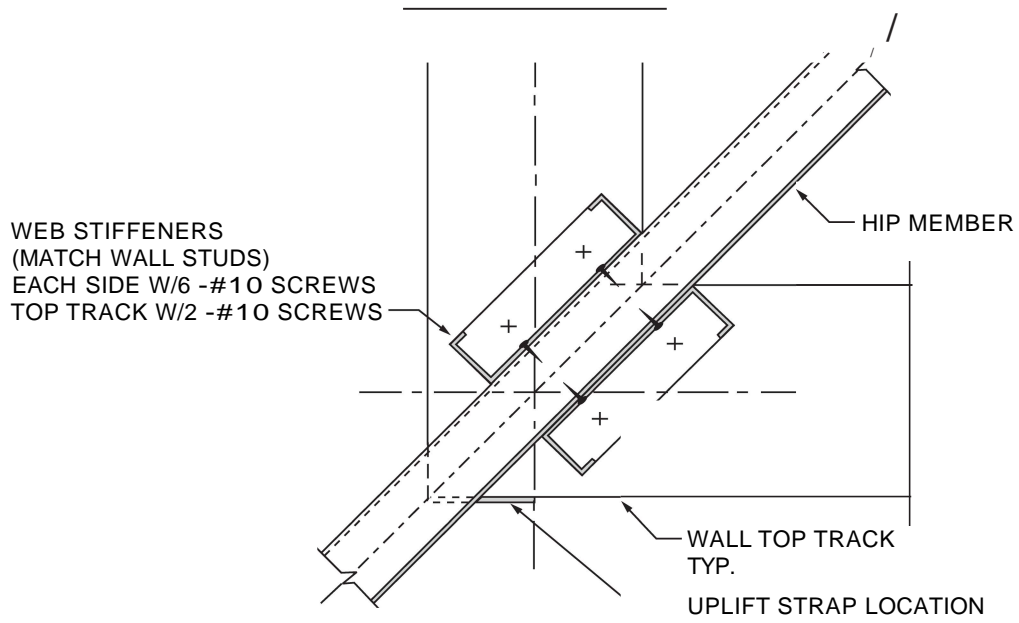
FIGURE R804.3.3.4(5) HIP MEMBER CONNECTION AT WALL CORNER
