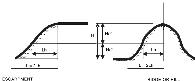
FIGURE R301.2.1.5.1(1) TOPOGRAPHIC FEATURES FOR WIND SPEED-UP EFFECT
