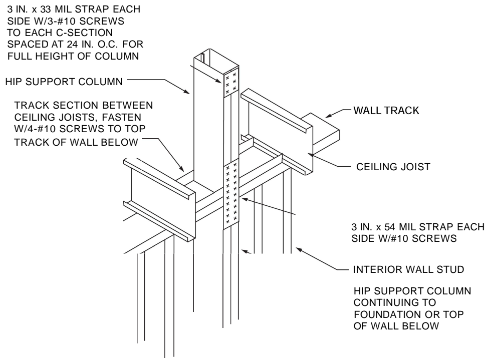
FIGURE R804.3.3.4(2) HIP SUPPORT COLUMN
