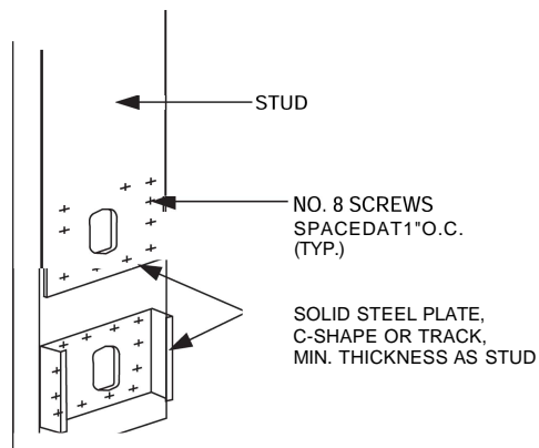
FIGURE R603.2.5.3 STUD WEB HOLE PATCH
