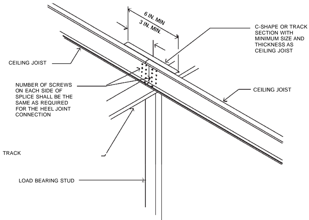
FIGURE R804.3.1.5 SPLICED CEILING JOISTS
