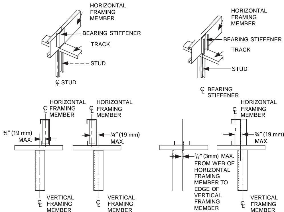
FIGURE R505.1.2 IN-LINE FRAMING
