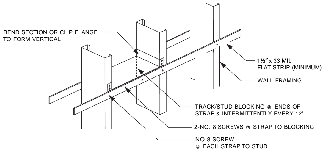
FIGURE R603.3.3(1) STUD BRACING WITH STRAPPING ONLY
