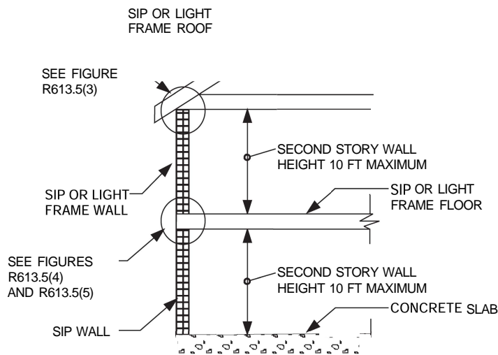
FIGURE R613.5(2) MAXIMUM ALLOWABLE HEIGHT OF SIP WALLS
