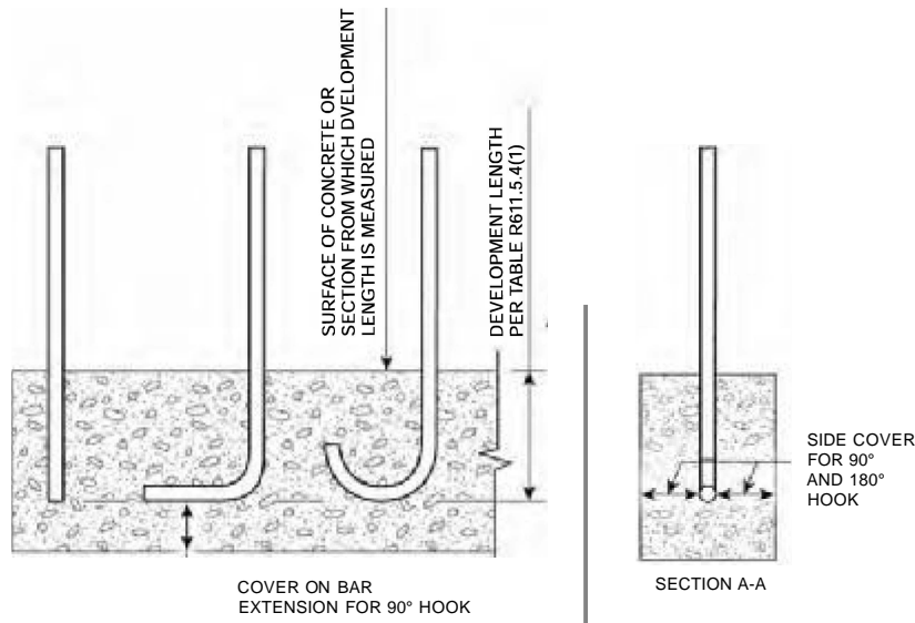
FIGURE R611.5.4(2) DEVELOPMENT LENGTH AND COVER FOR HOOKS AND BAR EXTENSION
