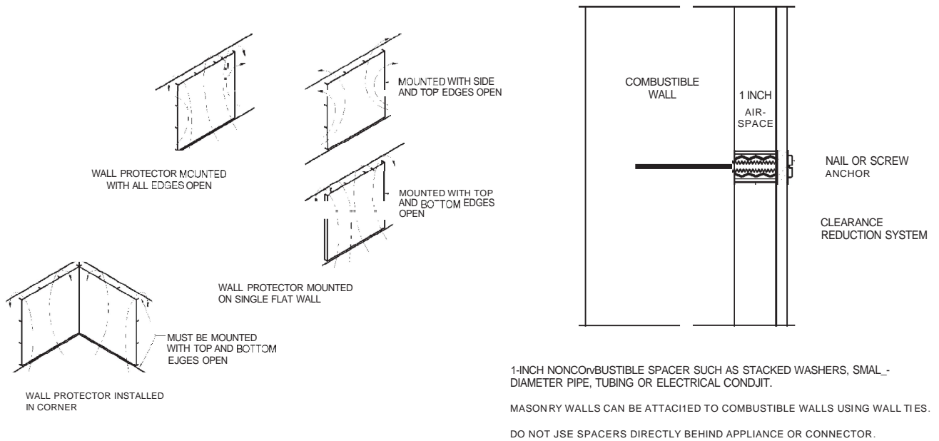
FIGURE G2409.2(2) [308.2(2)] WALL PROTECTOR CLEARANCE REDUCTION SYSTEM
