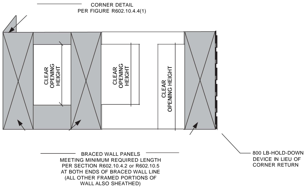
FIGURE R602.10.4.4(3) BRACED WALL LINE WITH CONTINUOUS SHEATHING WITHOUT CORNER RETURN PANEL
