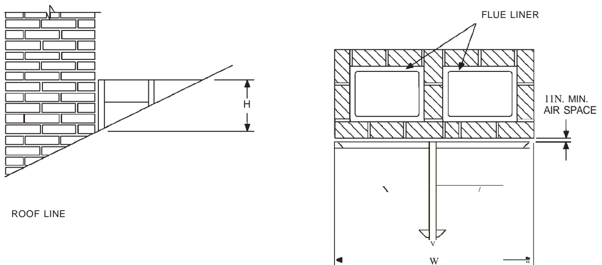
FIGURE R1003.18 CLEARANCE FROM COMBUSTIBLES
