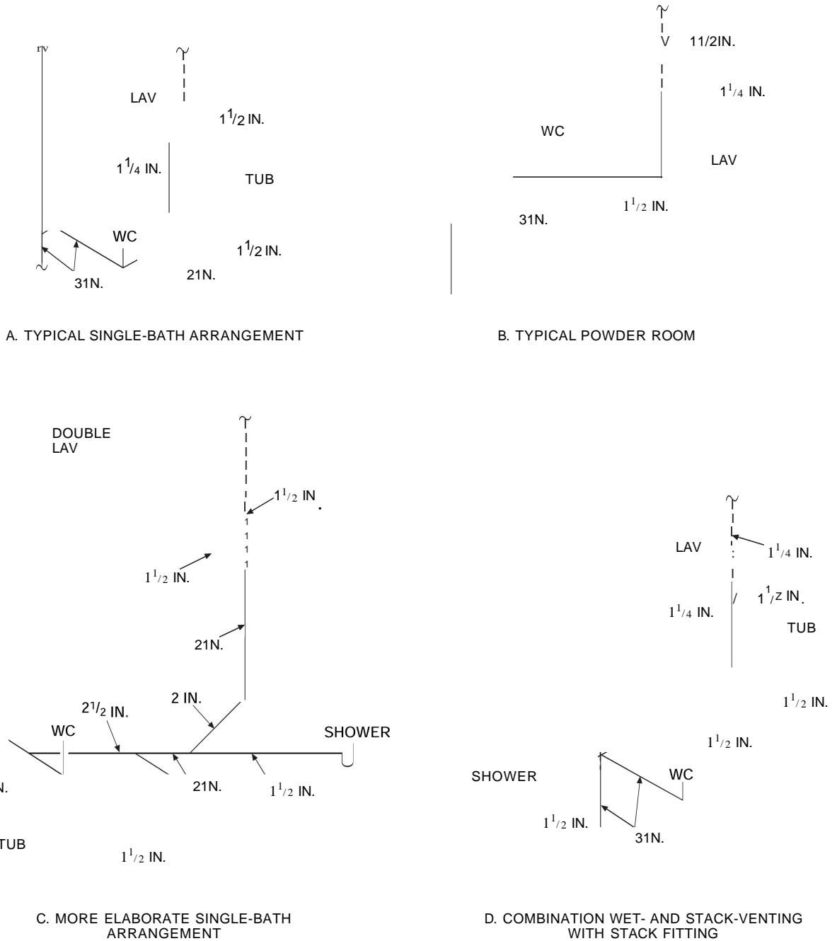
FIGURE N1 TYPICAL SINGLE-BATH WET-VENT ARRANGEMENTS
