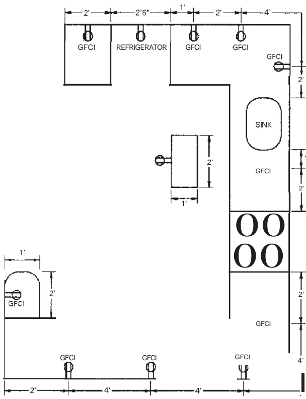
FIGURE E3901.4 COUNTERTOP RECEPTACLES
