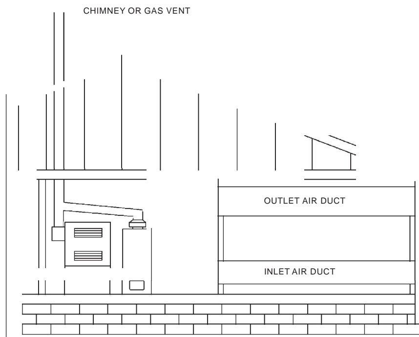
FIGURE G2407.6.1 (3) [304.6.1 (3)] ALL AIR FROM OUTDOORS (see Section G2407.6.1)
