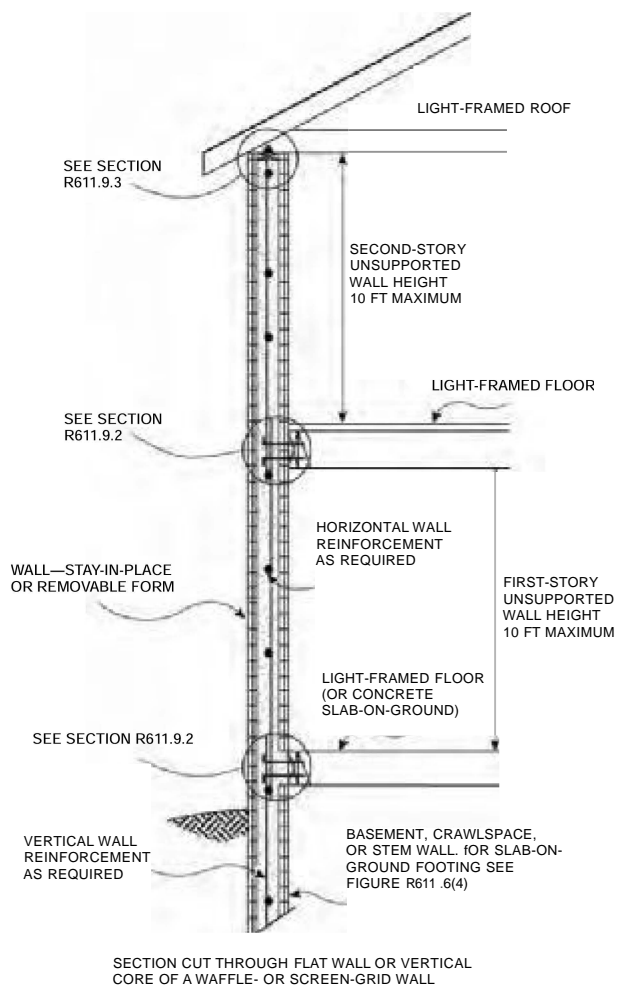
FIGURE R611.6(3) ABOVE-GRADE CONCRETE WALL CONSTRUCTION TWO-STORY
