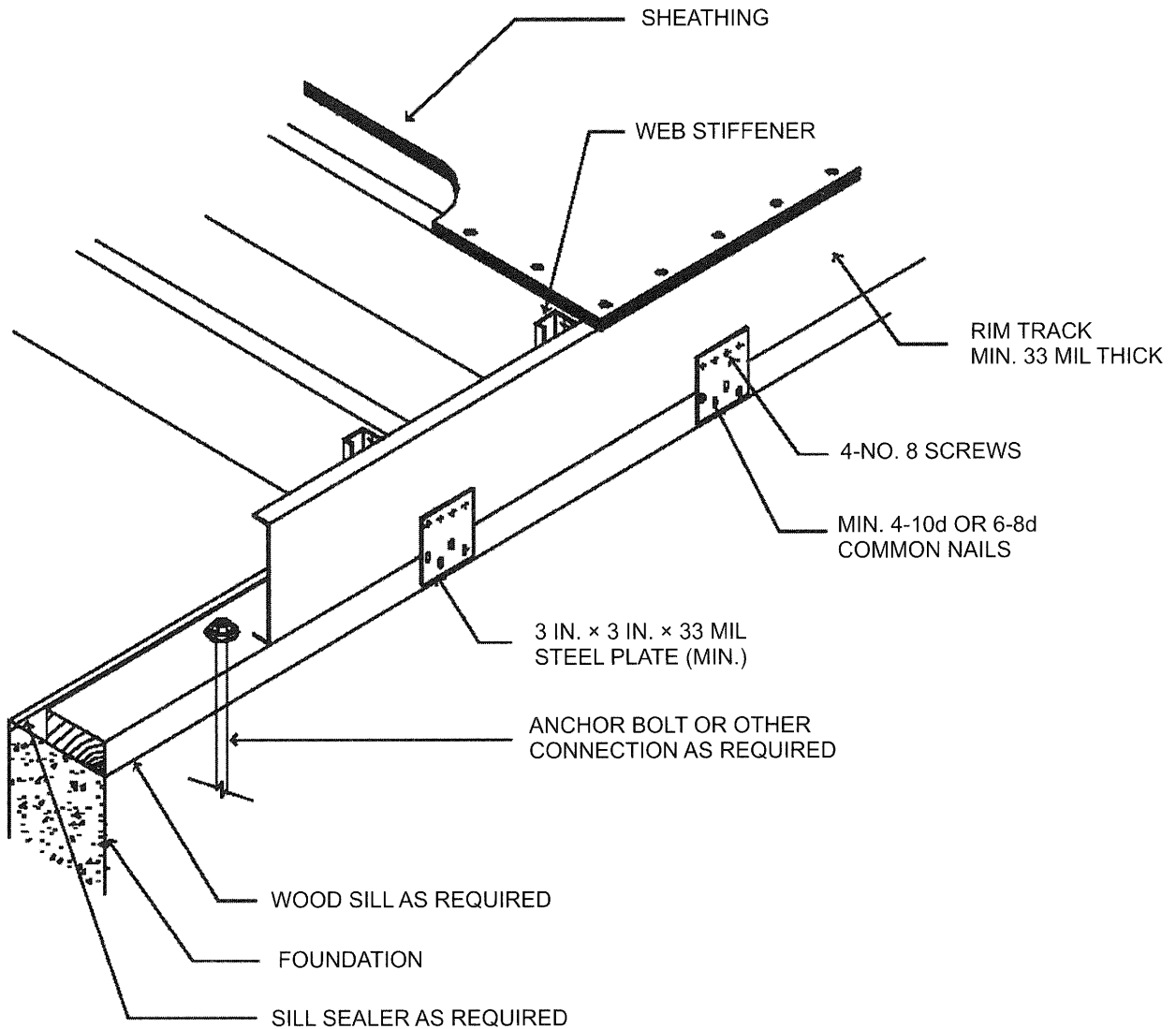
FIGURE R505.3.1(2) FLOOR TO WOOD SILL CONNECTION
