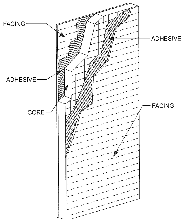
FIGURE R613.4 SIP WALL PANEL
