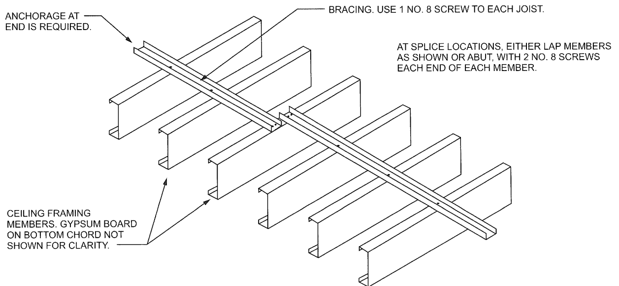
FIGURE R804.3.1.4(1) CEILING JOIST TOP FLANGE BRACING WITH C-SHAPE, TRACK OR COLD-ROLLED CHANNEL
