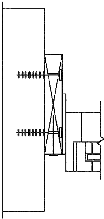
FIGURE R612.7.2(5) THROUGH THE FLANGE
