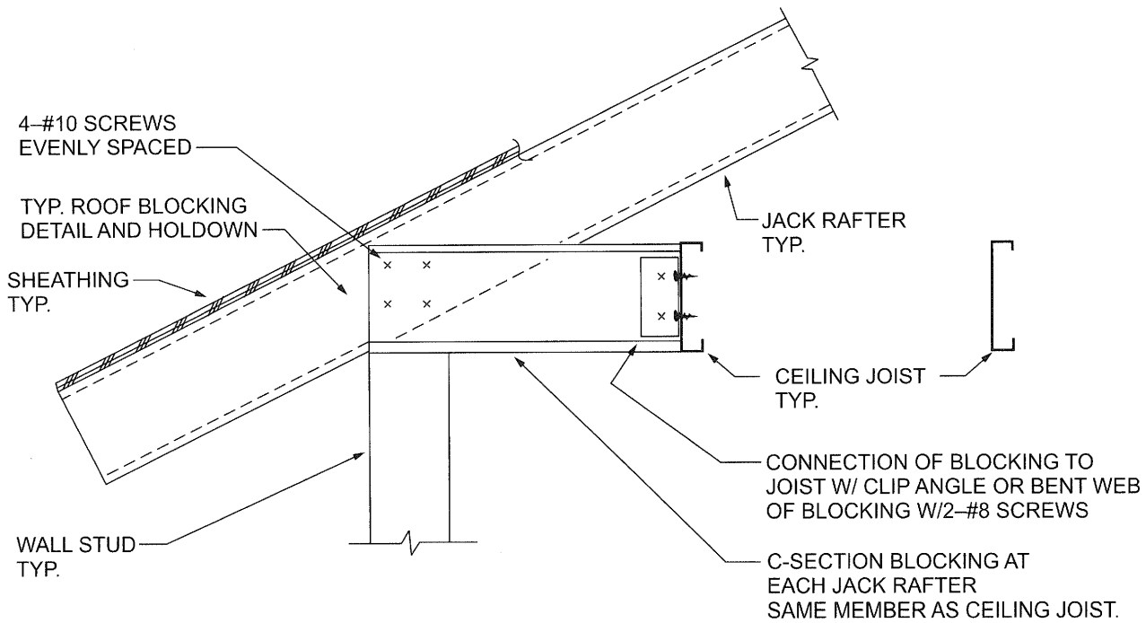
FIGURE R804.3.3.4(1) JACK RAFTER CONNECTION AT EAVE
