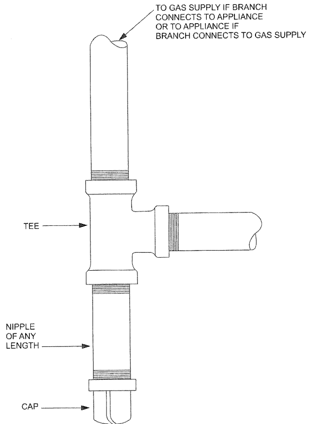
FIGURE G2419.4 METHOD OF INSTALLING A TEE FITTING SEDIMENT TRAP
