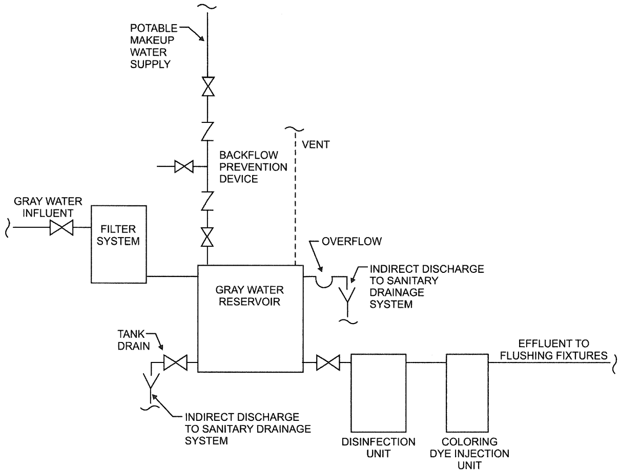
FIGURE P3009.1(1) GRAY WATER RECYCLING SYSTEM FOR FLUSHING WATER CLOSETS AND URINALS
