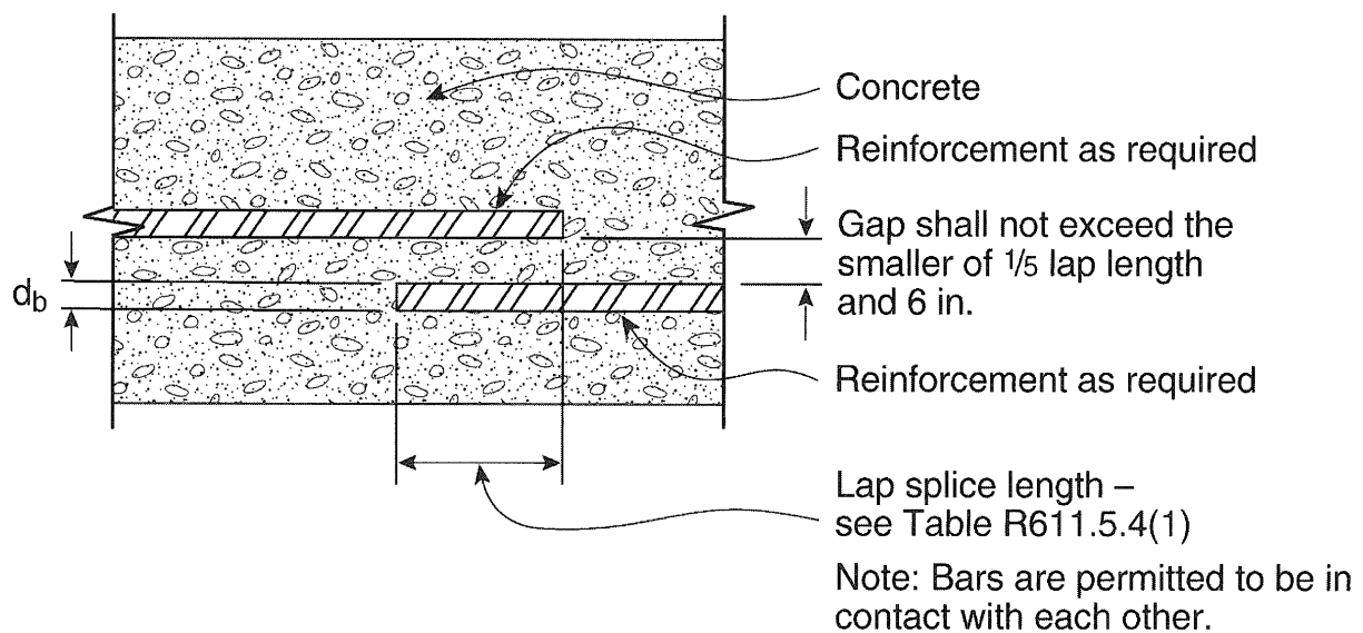
FIGURE R611.5.4(1) LAP SPLICES
