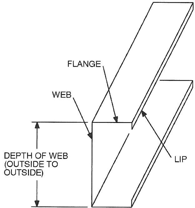
FIGURE R505.2(1) C-SHAPED SECTION
