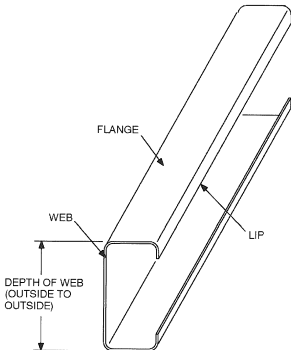
FIGURE R603.2(1) C-SHAPED SECTION
