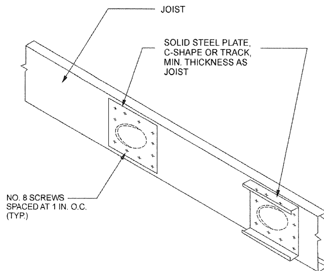
FIGURE R804.2.5.3 WEB HOLE PATCH
