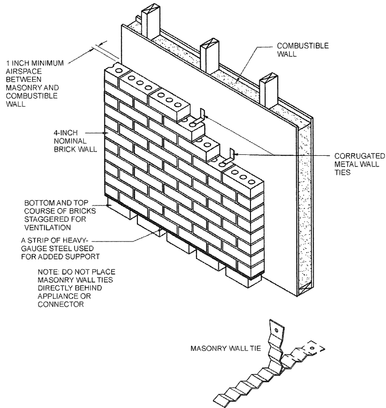
FIGURE G2409.2(2) [308.2(2)] WALL PROTECTOR CLEARANCE REDUCTION SYSTEM
