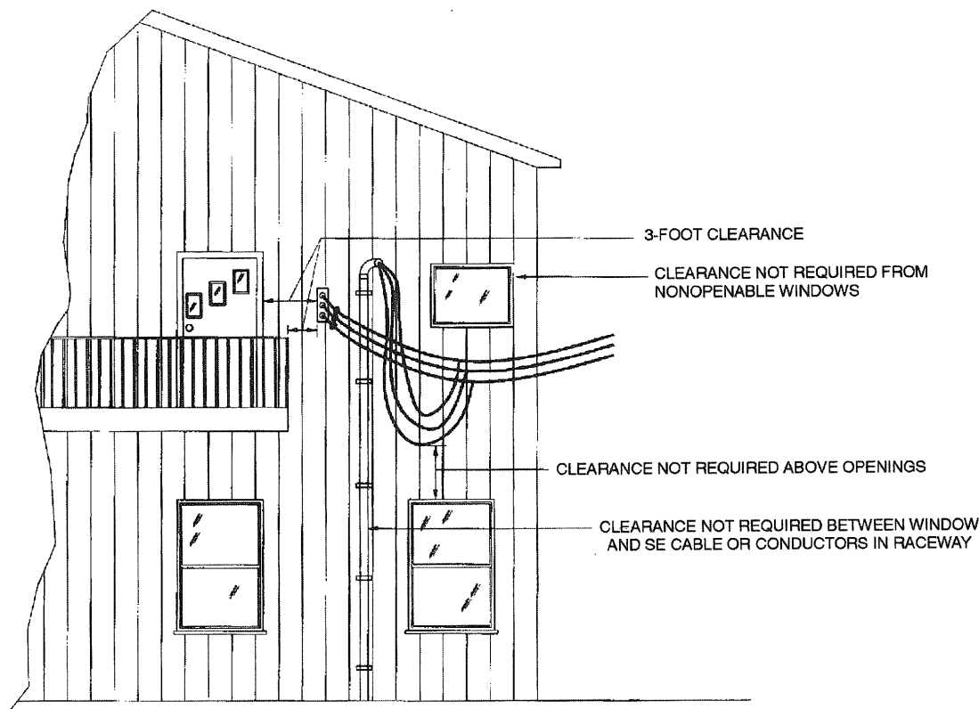
FIGURE E3604.1 CLEARANCES FROM BUILDING OPENINGS
