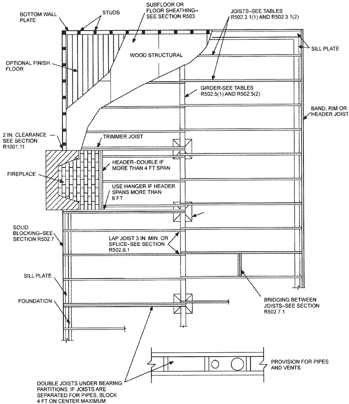
FIGURE R502.2 FLOOR CONSTRUCTION
