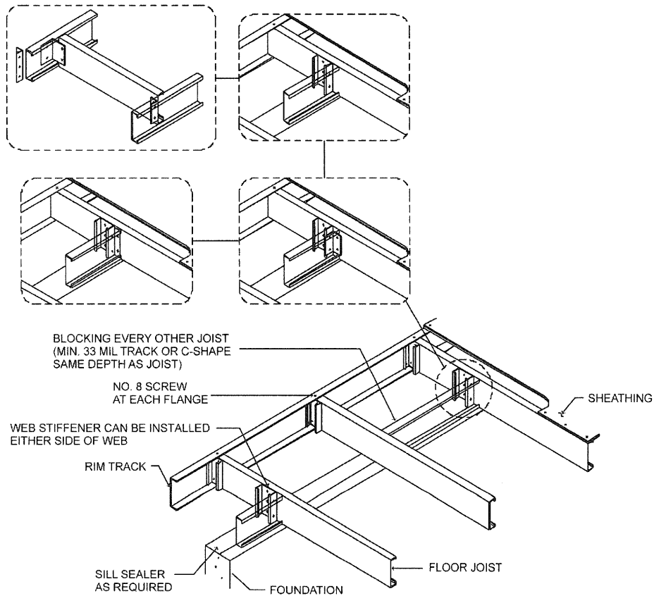
FIGURE R505.3.1(3) FLOOR TO FOUNDATION CONNECTION
