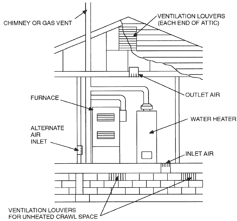
FIGURE G2407.6.1(1) [304.6.1(1)] ALL AIR FROM OUTDOOR-INLET AIR FROM VENTILATED CRAWL SPACE AND OUTLET AIR TO VENTILATED ATTIC (see Section G2407.6.1)
