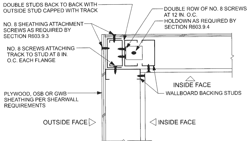
FIGURE R603.9.2 CORNER STUD HOLD-DOWN DETAIL
