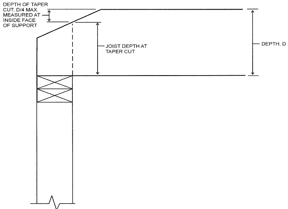
FIGURE R802.7.1.2 CEILING JOIST TAPER CUT
