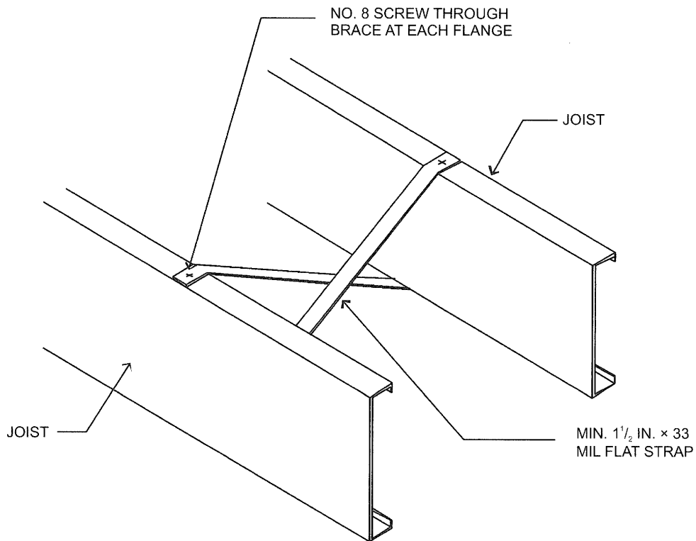
FIGURE R505.3.3.2(2) JOIST BLOCKING (STRAP)
