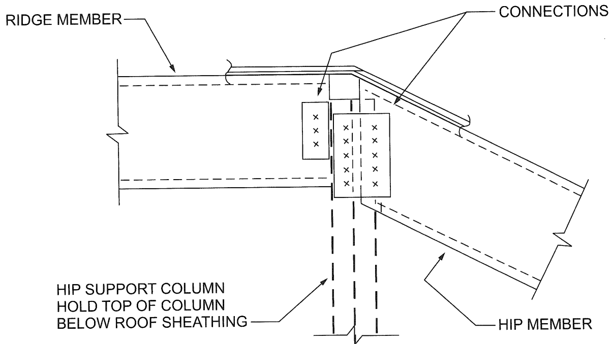
FIGURE R804.3.3.4(3) HIP CONNECTIONS AT RIDGE
