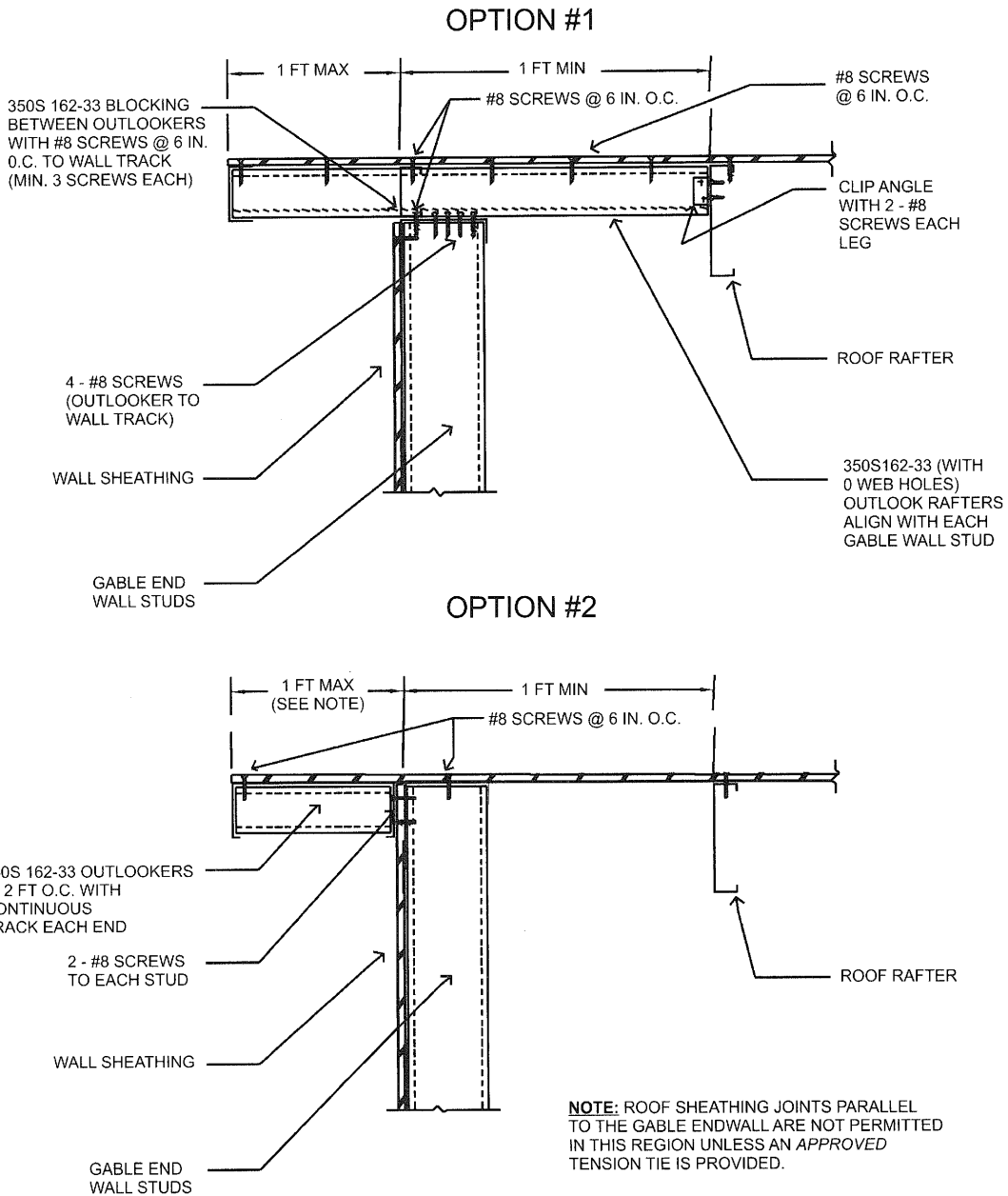
FIGURE R804.3.2.1.2 GABLE ENDWALL OVERHANG DETAILS
