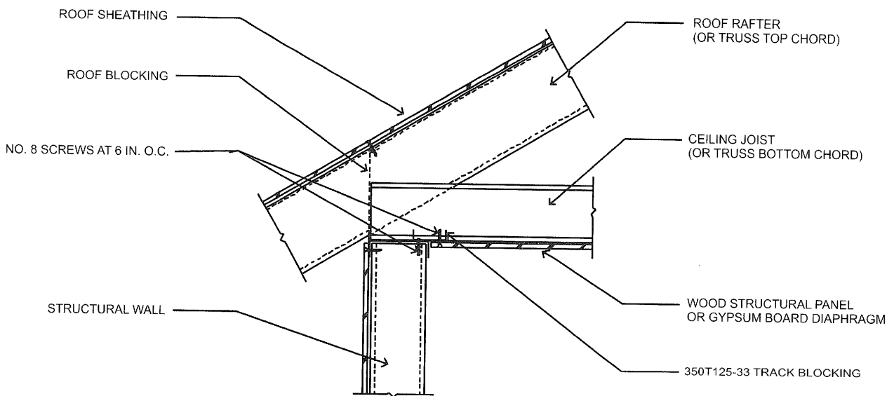
FIGURE R804.3.8(2) CEILING DIAPHRAGM TO SIDEWALL DETAIL
