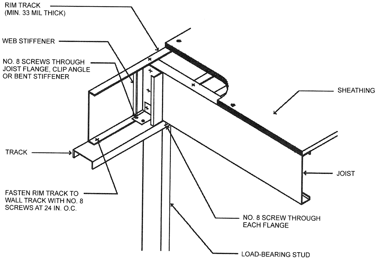
FIGURE 505.3.1(1) FLOOR TO EXTERIOR LOAD-BEARING WALL STUD CONNECTION
