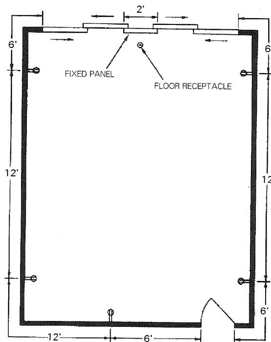
FIGURE E3901.2 GENERAL USE RECEPTACLE DISTRIBUTION
