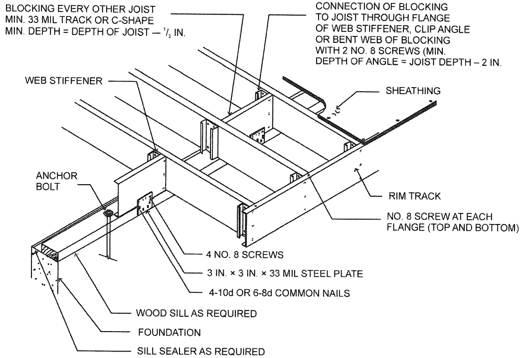
FIGURE R505.3.1(5) CANTILEVERED FLOOR TO WOOD SILL CONNECTION
